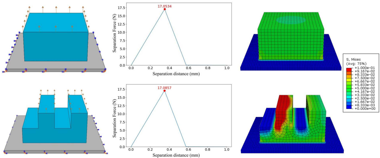
Figure 5. Comparison of zero-gravity simulation results for two models with identical cross-sections but different 3D shapes.
