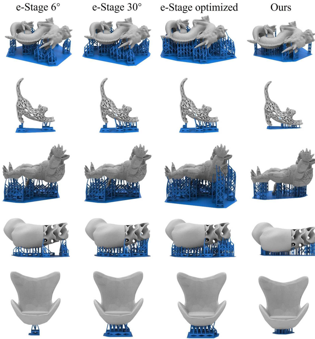
Figure 21. Comparison of support structures. From left to right, the images display support structures generated by e-Stage for overhang angles of 6^\circ , 30^\circ , and print-optimized angles that ensure fabrication success, respectively. The last column shows the results produced by our method.
