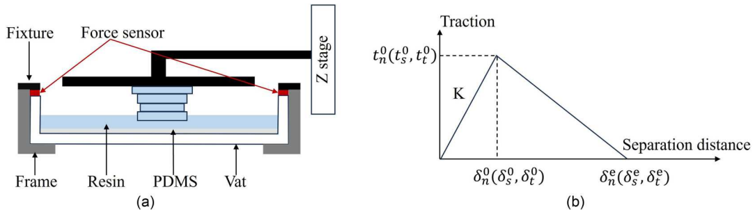
Figure 12. Schematic of the force sensor setup and traction-separation response. (a) Illustration of the force sensor apparatus. (b) Demonstration of parameter extraction for Equation (4) based on the relationship between separation force and displacement.
