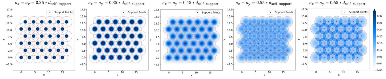
Figure 16. Stress field distributions with varying \sigma_x and \sigma_y values ( 0.25 - 0.65 \times \ell_{Gi}d_{\text{self-support}} ).
