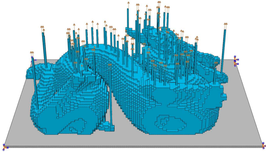
Figure 7. Simulation boundary conditions: A uniform velocity is applied to the top endpoint of the support in the positive Z-axis direction, along with the bottom of the separation film.
