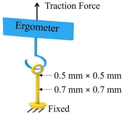
Figure 14. Schematic diagram of the support breakage threshold test. The yellow test model was printed and stretched using a blue force gauge until a fracture occurred. The breakage threshold was measured as 1.2 N for a cross-section of 0.5 \text{ mm} \times 0.5 \text{ mm} .
