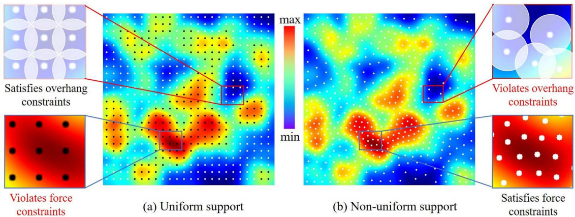
Figure 3. Support distributions governed by overhang constraints and traction force. A random stress field is visualized using a color gradient from blue (low stress) to red (high stress). (a) In the uniform support distribution, insufficient supports in high-stress regions violate force constraints, risking structural failure. (b) In the non-uniform distribution, supports in low-stress regions fail to satisfy overhang constraints, as circles with maximum overhang radius centered at supports cannot fully cover the overhang area.
