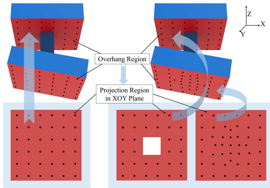
Figure 11. Schematic illustration of overhang region mapping methods. (a) Uniform support approach [14] maps multiple overhang regions to identical XOY plane locations. (b) Our non-uniform approach maps overhang regions to distinct locations for force-based support optimization before inverse mapping.
