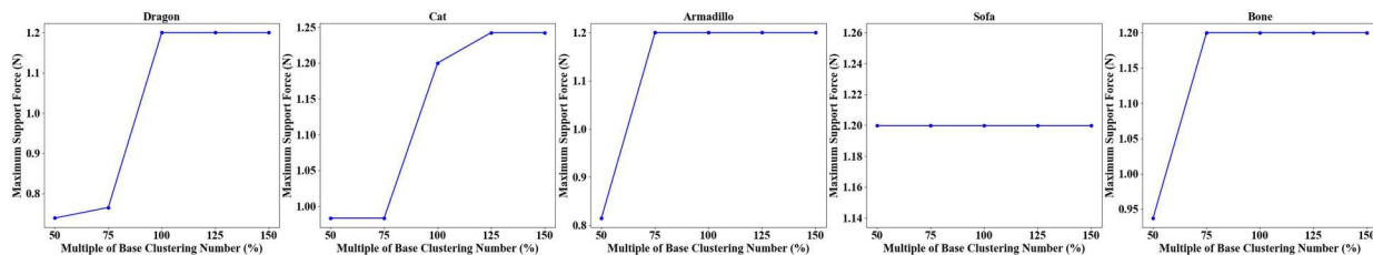
Figure 20. Maximum support forces under different clustering ratios (50%–150% of base clustering number) for five test models.
