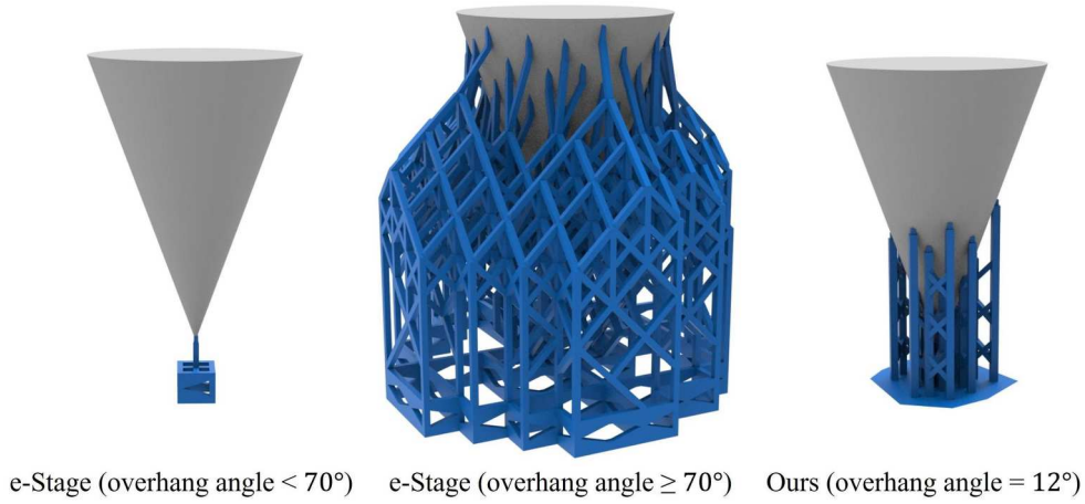
Figure 9. Comparison of support structures for a conical model.
