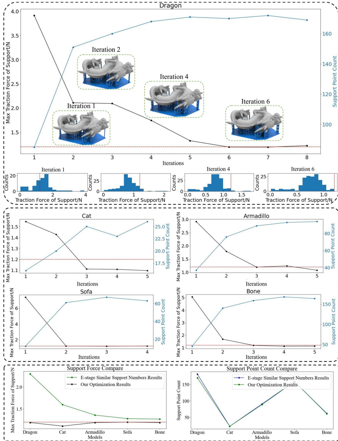
Figure 19. Iterative analysis process showing support distribution, traction forces and 3D support results for various models.
