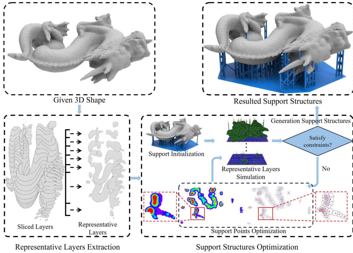
Figure 4. Adaptive support algorithm pipeline. Given a 3D shape and printing parameters, the Representative Layers Extraction module slices the model, clusters layers by image similarity, and selects the maximum load layer from each cluster for simulation. In the Support Structures Optimization phase, initial supports are generated to satisfy overhang constraints, and then support points are optimized iteratively until all constraints are met. The final support structures are produced based on the optimization results.
