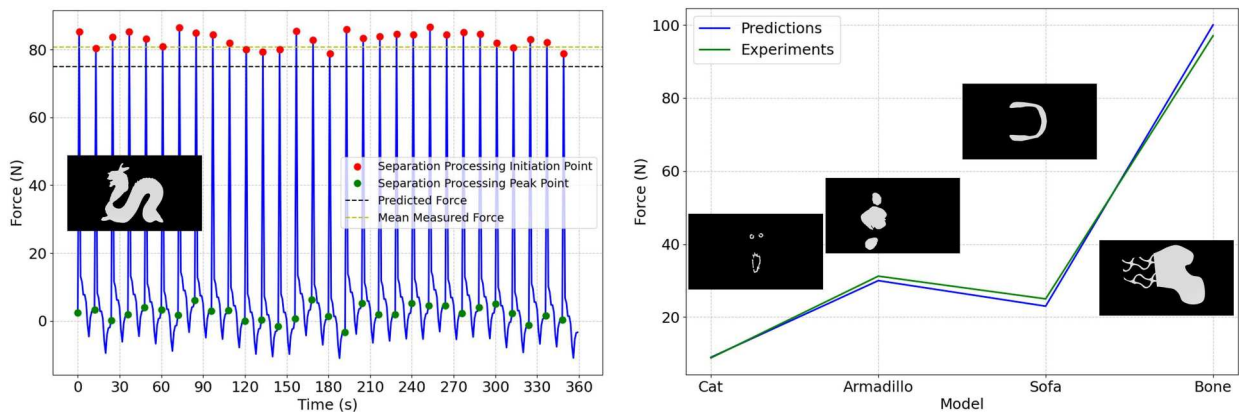
Figure 23. Comparison between MLP predictions and mean experimental forces.
