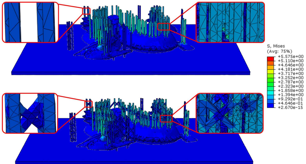
Figure 8. Stress analysis comparing support structures with and without truss reinforcement. The nearly identical stress distributions in support rods across both configurations validate the truss-free simulation approach, while the truss structure exhibits stress levels an order of magnitude lower than its connected supports.
