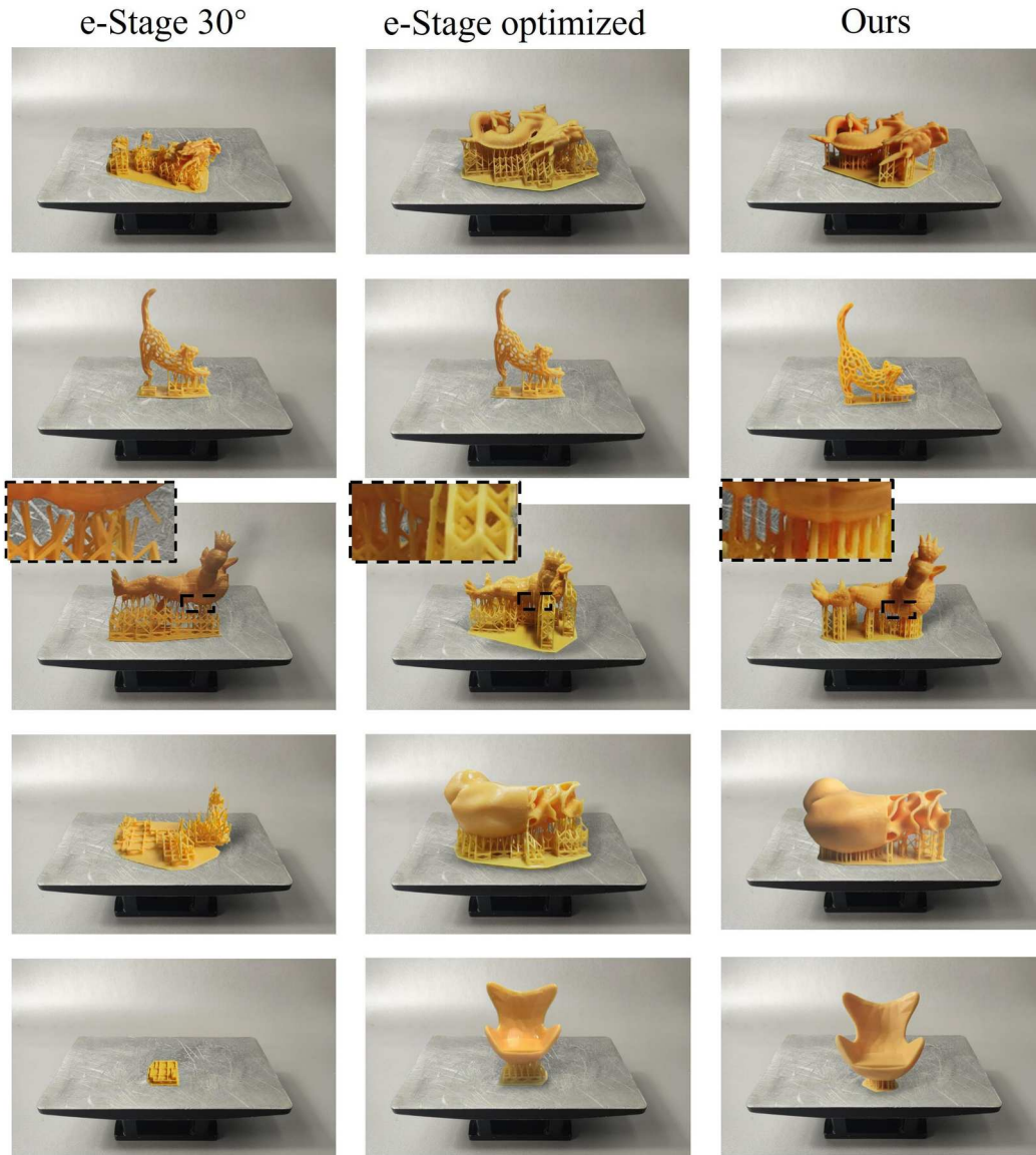
Figure 22. Comparison of printing results.
