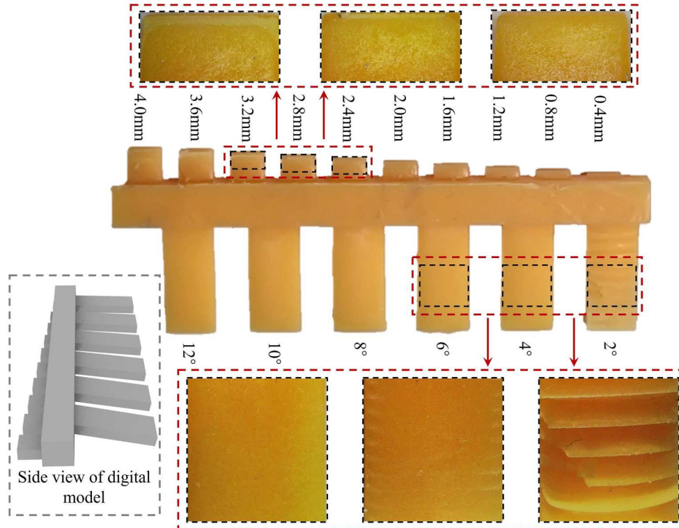
Figure 15. Experiment determining the maximum overhang distance and angle.
