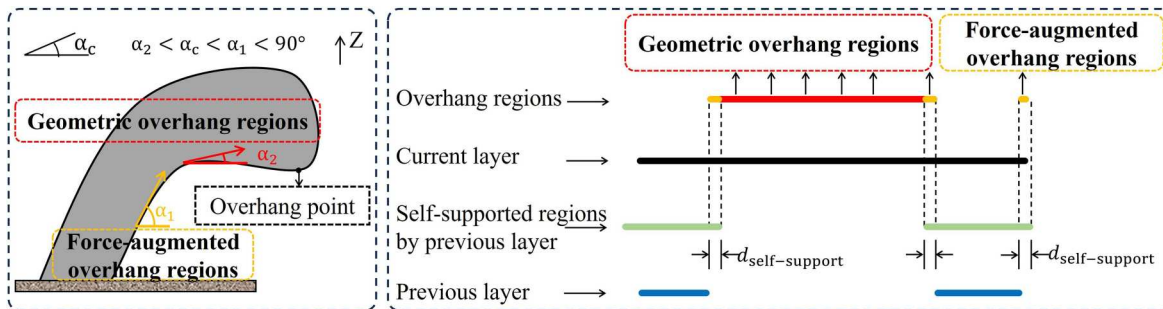
Figure 10. Determination of geometric overhang and force-augmented overhang regions in mesh (left) and slice (right) representations.
