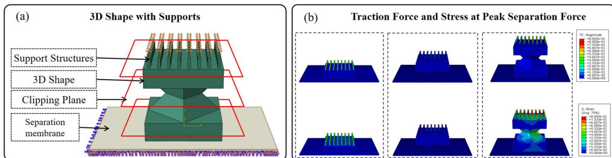
Figure 2. The schematic demonstrates the separation process for a shape with supports across different layers.
