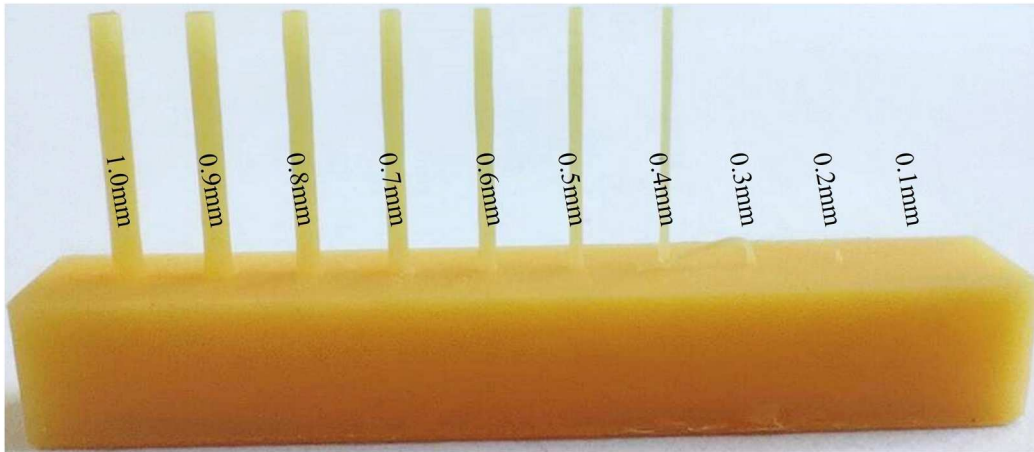
Figure 13. Experiment determining the minimum side length of the support.
